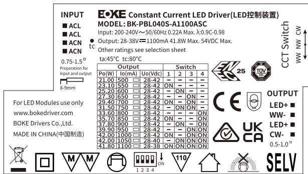
BK-PBL040S-A1100ASC
