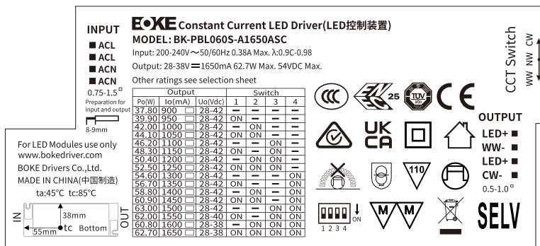
BK-PBL060S-A1650ASC
