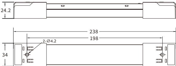
SKL030S-AHB/SKL040S-AHB/SKL050S-AHB
