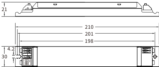
SKL030S-AHB/SKL040S-AHB/SKL050S-AHB
