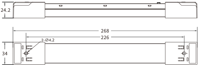
SKL060S-AHB/SKL080S-AHB
