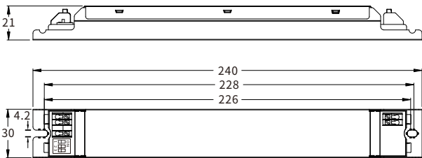
SKL060S-AHB/SKL080S-AHB
